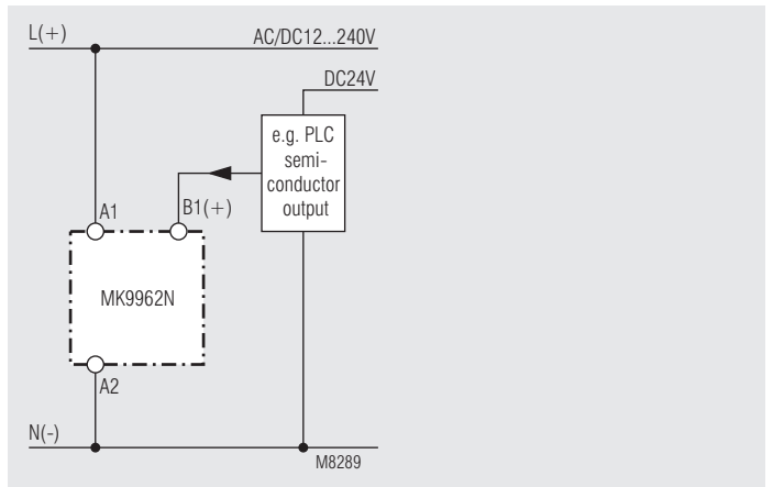
Connection with 2 different control voltages
