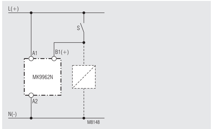
Control with parallel connected load
